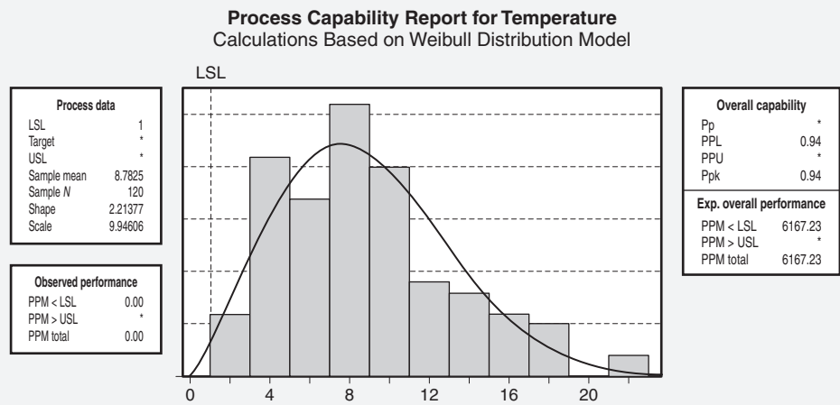
Figure 19.4 Nonnormal process capability analysis based on the Weibull distributiona.
