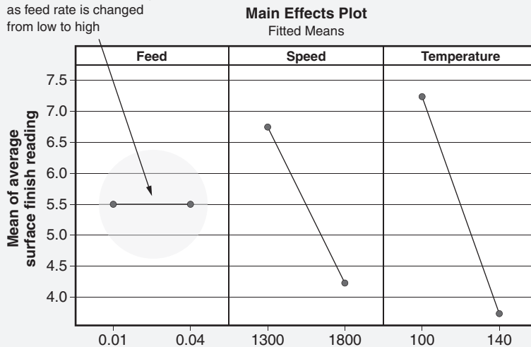
Figure 24.3 Graph of the main effects for Example 24.3.
