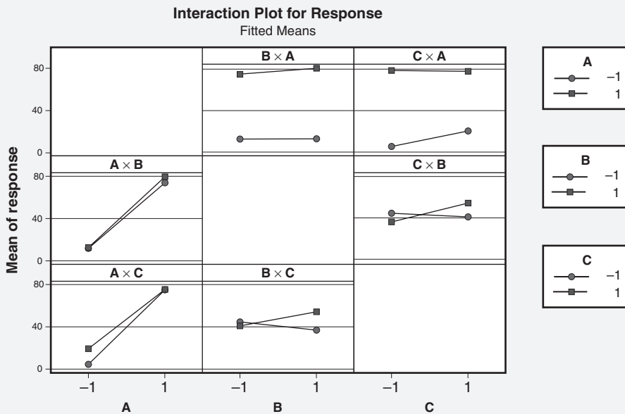
Figure 24.8 Interaction plot for the initial model.
