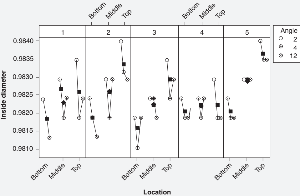
Figure 20.16 Multi-vari chart of data from Table 20.10.
