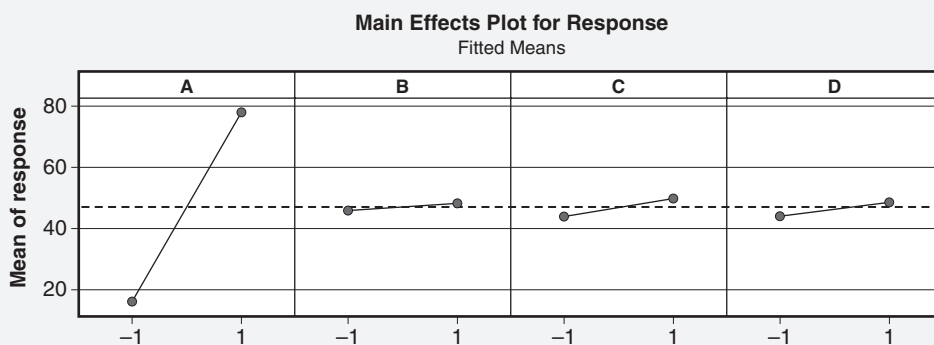
Figure 24.7 Main effects plot for the initial model.
