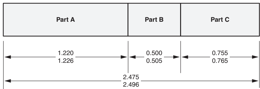
Figure 33.5 Conventional stack tolerance dimensioning.
